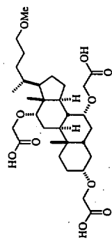
3a (CD 3 OOD/CD 3 OD/CDCl 3 , 500 MHz)
